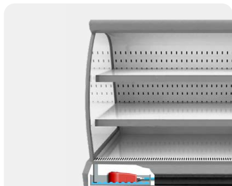
Pump inside the tray condensate inlet on the bottom of the pump
