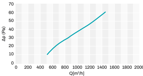
SIDE COLLAR DN. 250 mm (DIFF. 520 x 520 mm)
