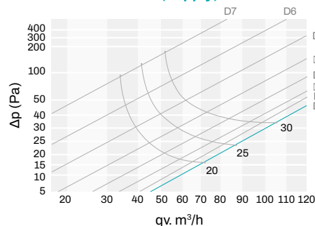
CANOVA Ø125 (supply)
