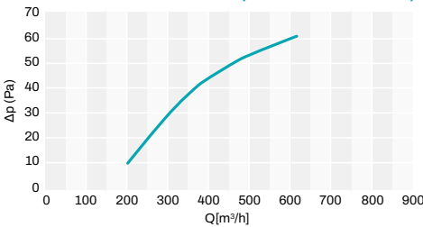
SIDE COLLAR DN. 150 mm (DIFF. 370 x 370 mm)
