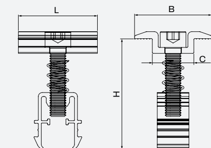
DIMENSIONS [mm]
