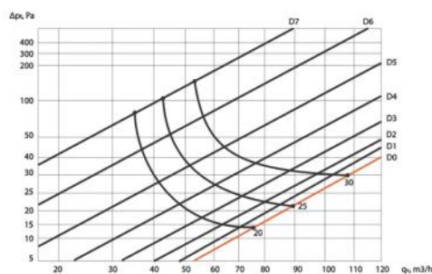
Canova Ø 125 (mandata / supply air)
